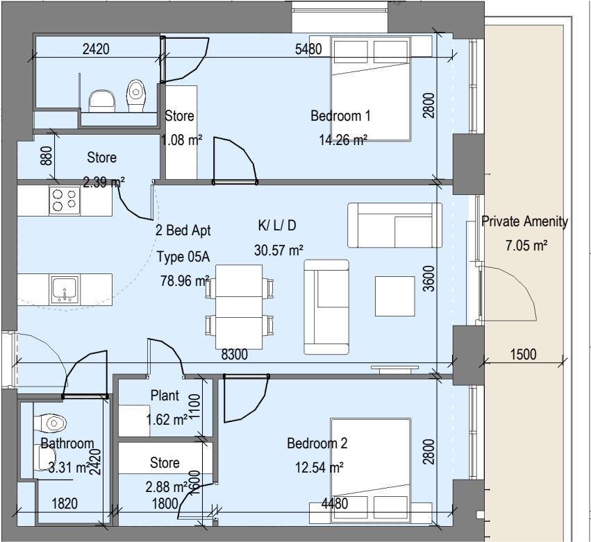
1 2 Bed Apt - Type 05A
