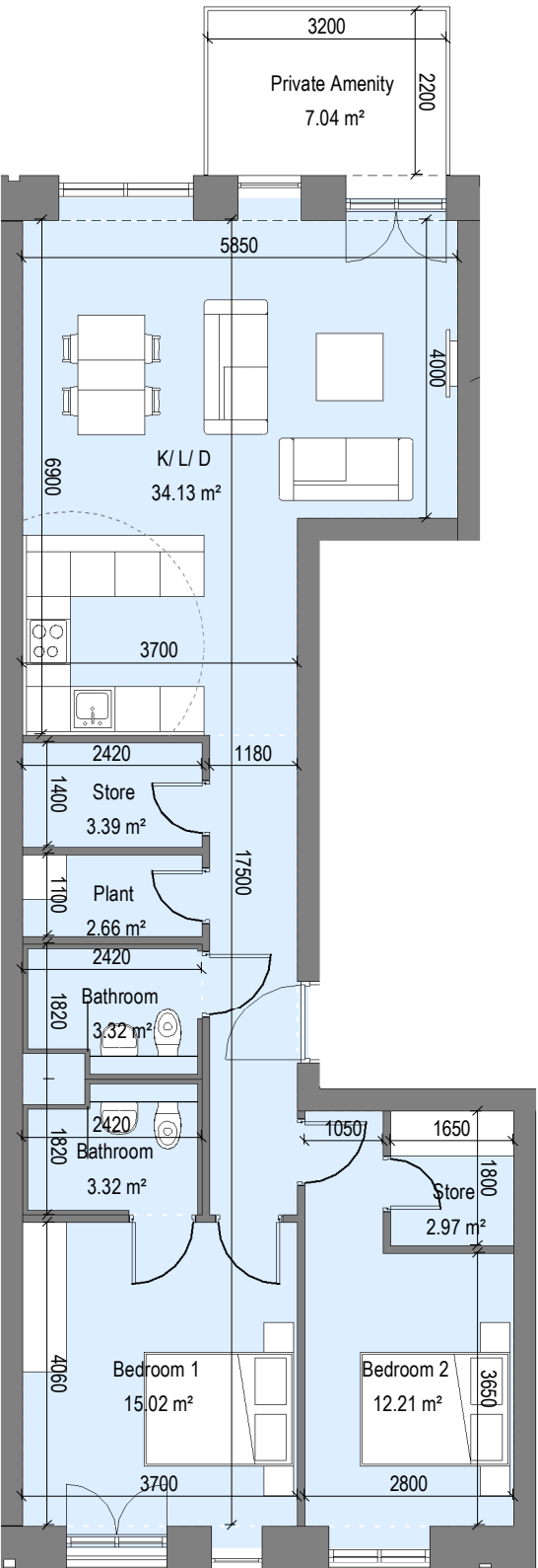
1 2 Bed Apt - Type 06
