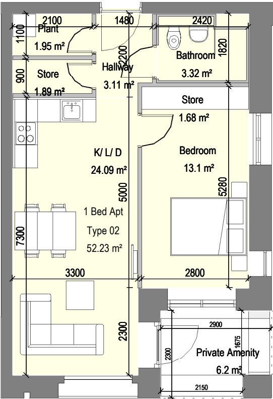
2 1 Bed Apt - Type 02
