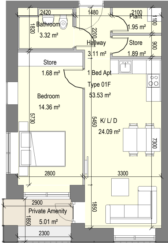
1 1 Bed Apt - Type 01F
