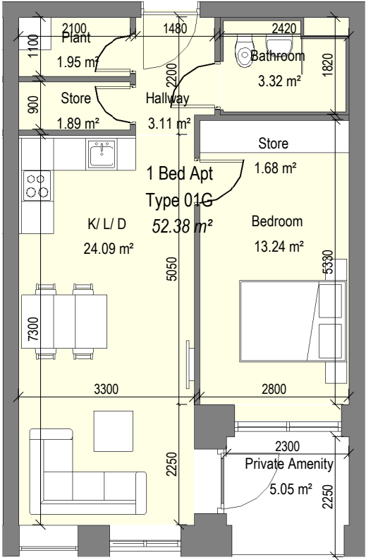
1 1 Bed Apt - Type 01G
