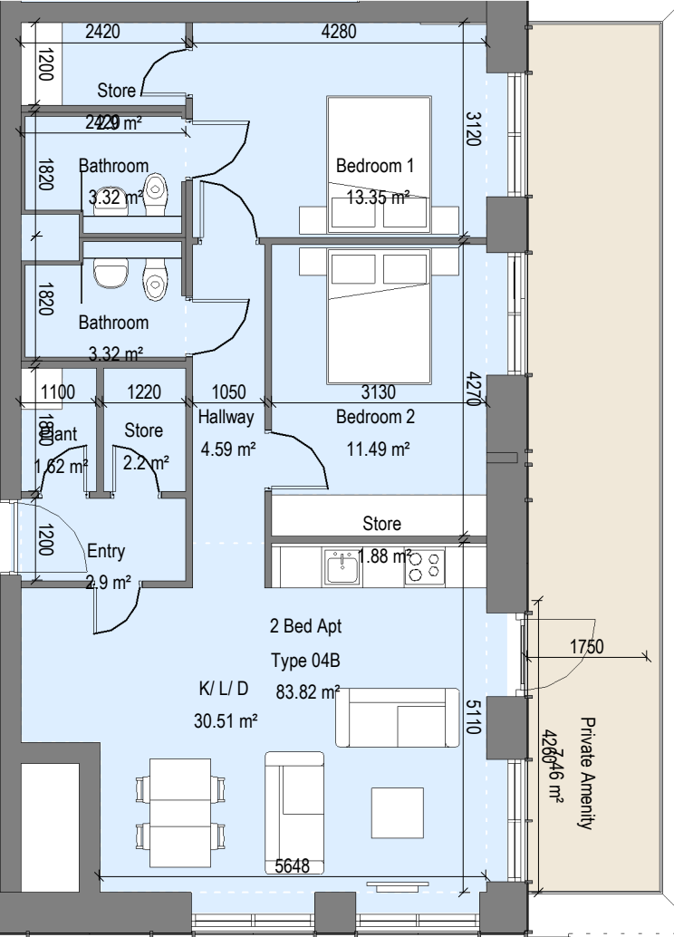
1 2 Bed Apt - Type 04B
