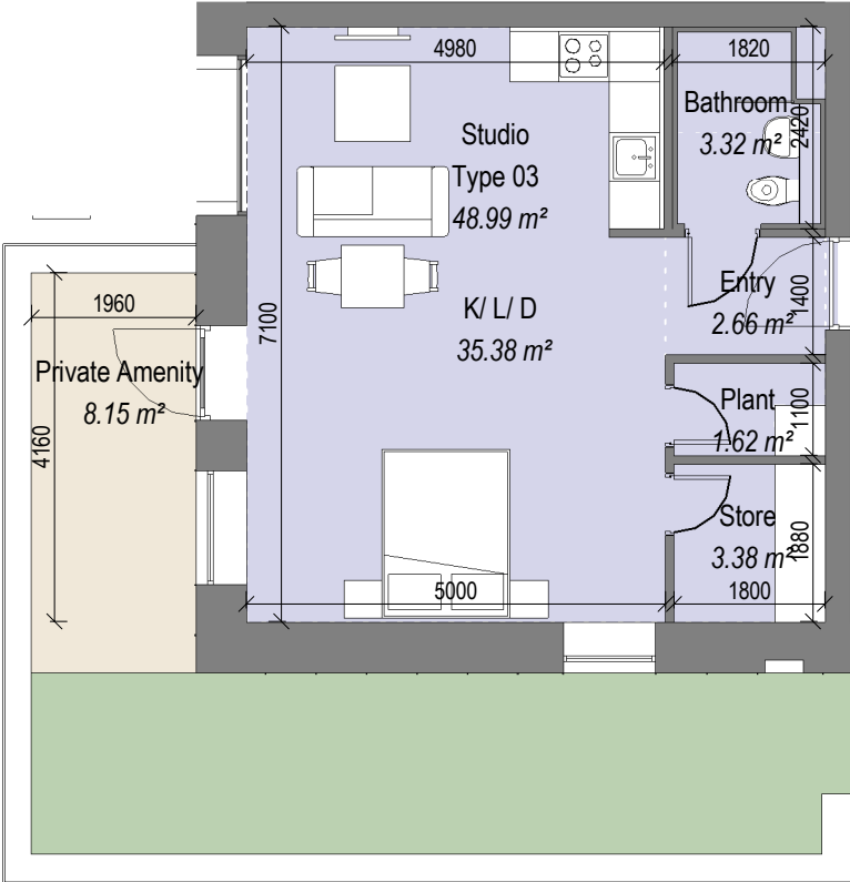
1 Studio - Type 03
