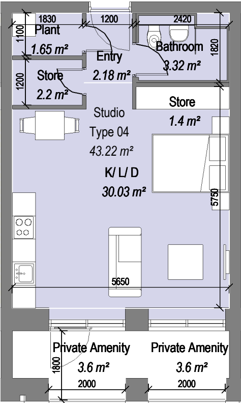
1 Studio - Type 04
