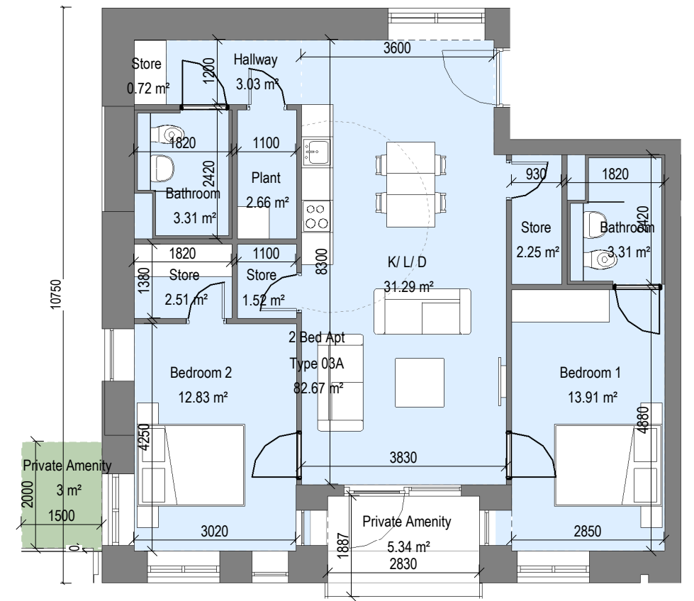
1 2 Bed Apt - Type 03A
