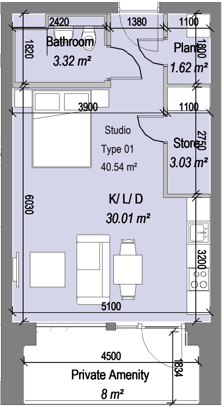
1 Studio - Type 01
