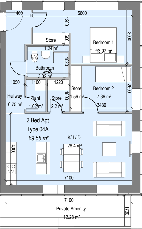
1 2 Bed Apt - Type 04A
