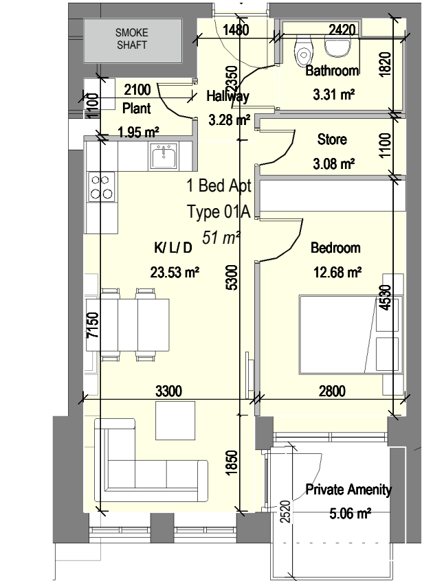
1 1 Bed Apt - Type 01A
