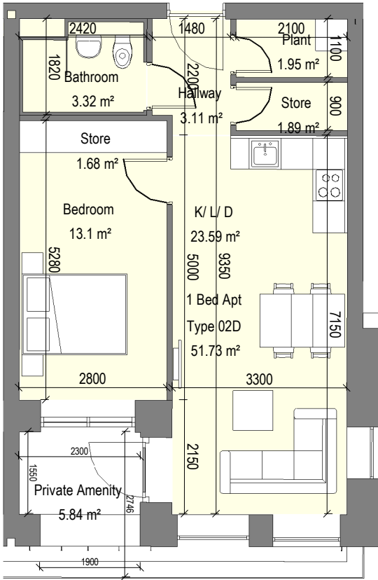
1 1 Bed Apt - Type 02D
