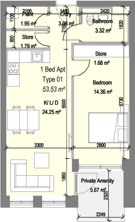
1 1 Bed Apt - Type 01
