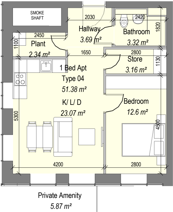
1 1 Bed Apt - Type 04
