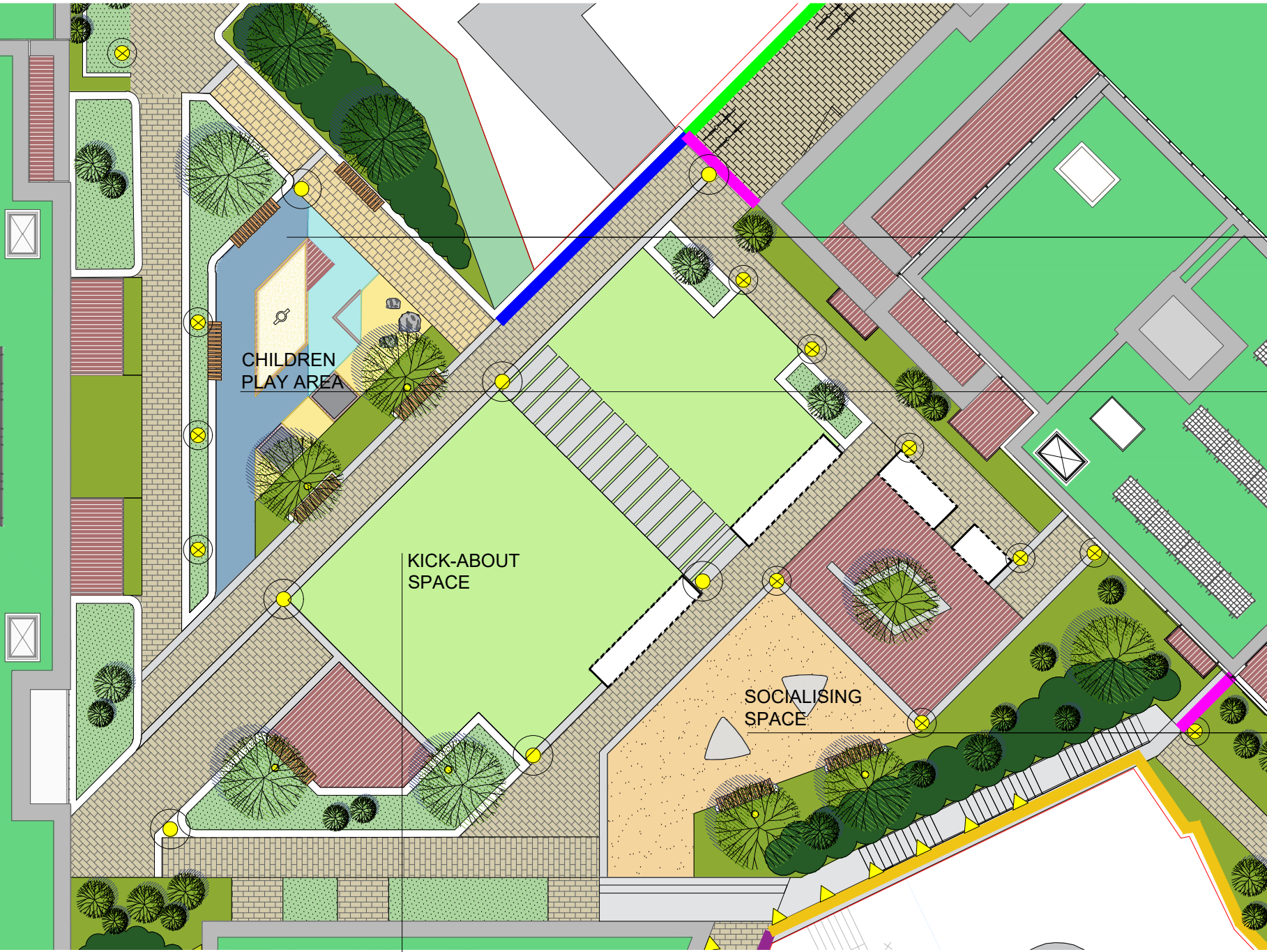
BLOWN-UP COURTYARD MASTERPLAN 1:200 @ A3
