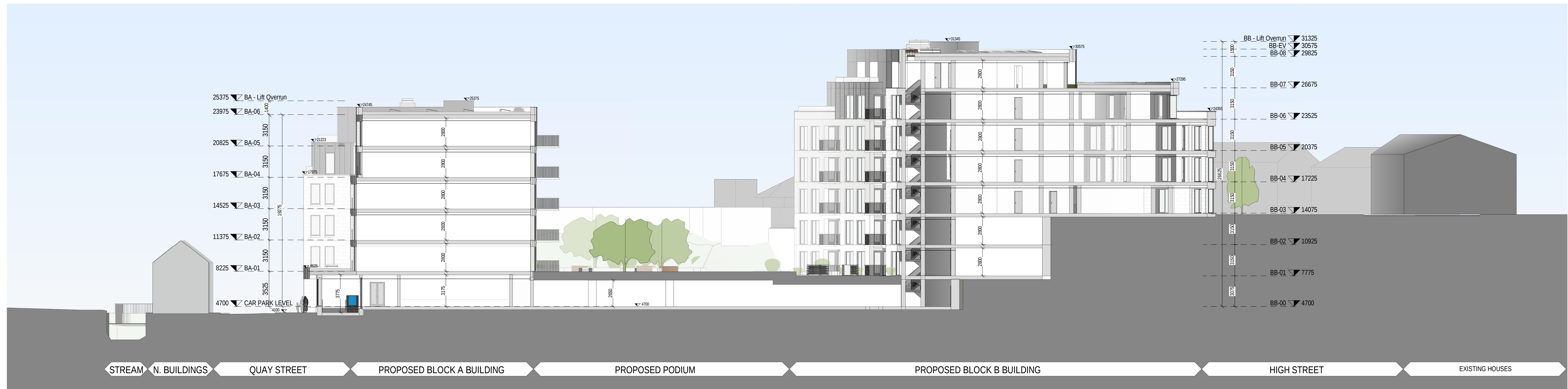
3 Contextual Section AA 1 : 200
