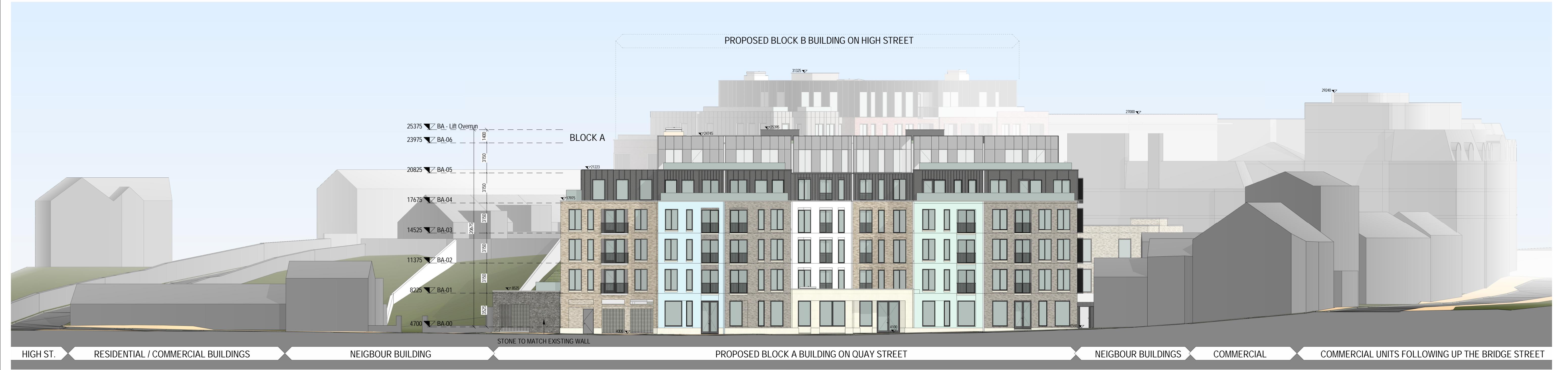
1 CONTEXTUAL ELEVATION QUAY STREET 02 1 : 200
